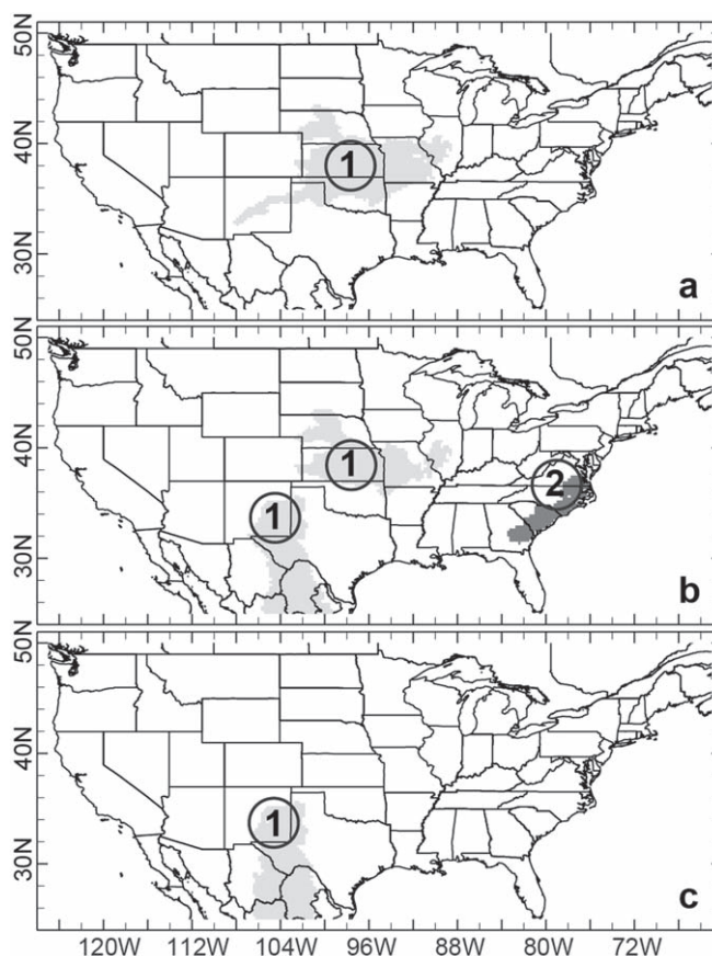
Figure 1. Contiguous heat wave regions identified in NARR when the daily maximum temperature exceeds the 95th percentile for 3 or more consecutive days. Panel (a) is for 2 August 1980 where a single heat wave event is identified in the central US. Panel (b) for 3 August shows the first heat wave breaks into two sub-regions while a second heat wave emerges along the southeast coast. In panel (c) only the remnants of the first heat wave region persist.
